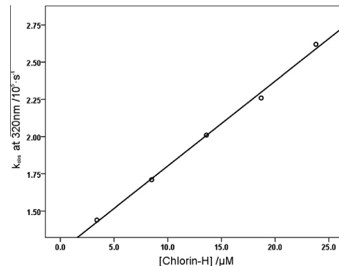
Figure 4. Dependence of the triplet decay rate constant k_{\text{obs}} on concentration at 320 nm for Chlorin-H.
