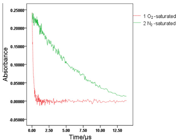
Figure 3. Transient time profile observed at 440 nm in \text{N}_2 -saturated solution and \text{O}_2 -saturated solution. (1) In \text{O}_2 -saturated solution (8.5 \mu\text{M} ). (2) In \text{N}_2 -saturated solution (8.5 \mu\text{M} ).
