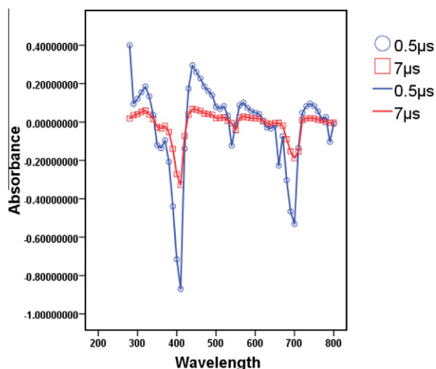
Figure 2. Transient absorption spectra recorded after 355 nm laser flash photolysis of Chlorin-H in \text{N}_2 -saturated \text{CH}_3\text{CN} (8.5 \mu\text{M} ). (a) At 0.5 \mu\text{s} . (b) At 7 \mu\text{s} .
